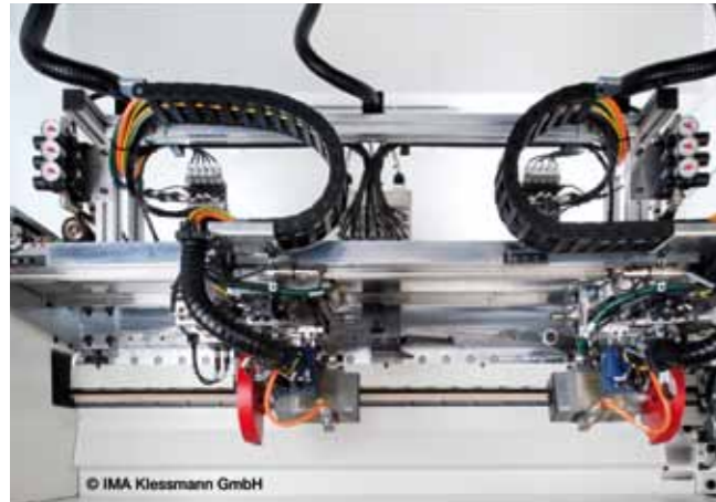
triflex® R in einem Kapp-Aggregat triflex® R in a machine for wood working industry
